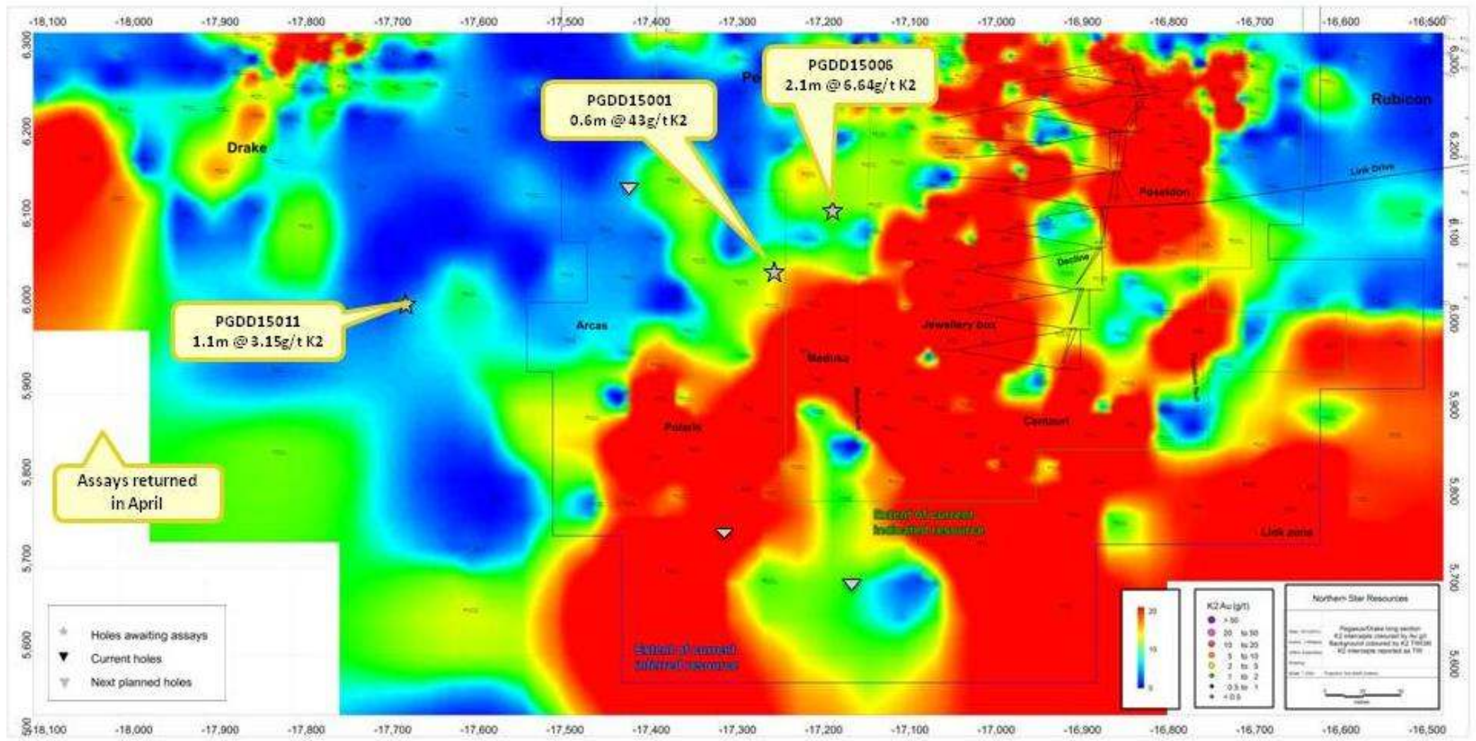
Figure 6. Pegasus K2 Long section
